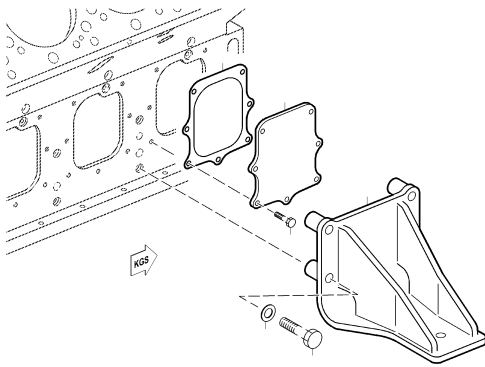
SHPG STAND + ENG SKID MTG 16V4000 C23/S8 UPC.06Q01 0201
