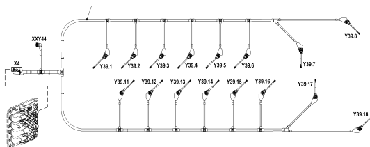
ADEC HARNESS + SENSORS 16V4000 X00035192 UPC.06N04 4510
