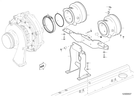
AIR SYSTEM INTAKE NECK 16V4000 C23 X0001 UPC.06M03D0006
