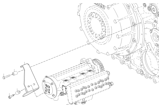
PUMP FUEL BRACKET W/TRUNION S4000 C23/S8 UPC.06M04A0005
