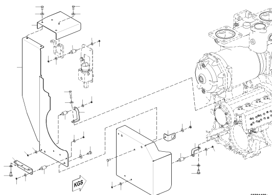
HARNESS GUARD PLATE C23 16V4000 X0003893
