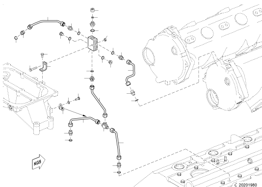
COOLANT VENT SYSTEM 16V4000 C23 X0001935 UPC.06K03 2700
