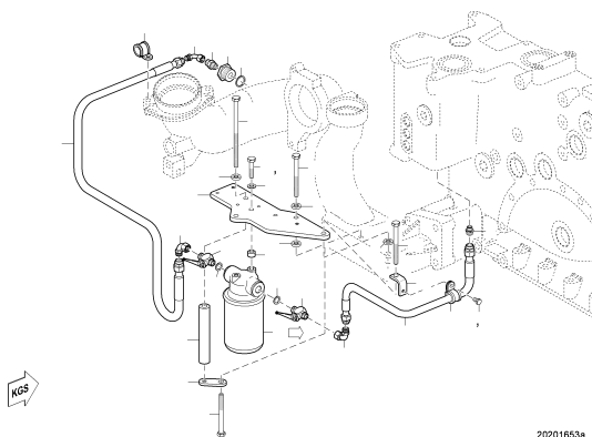
FILTER CLNT ENGINE S4000 X00023104 UPC.06K02C0002
