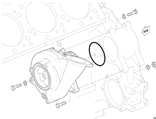
PUMP WAT HI TEMP S4000 XS526200.00020 UPC.06K02 0508
