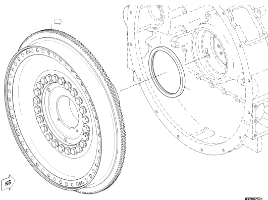
FLYWHEEL ASM ADEC 2 PIECE S4000-03 X0001 UPC.06C03 1600
