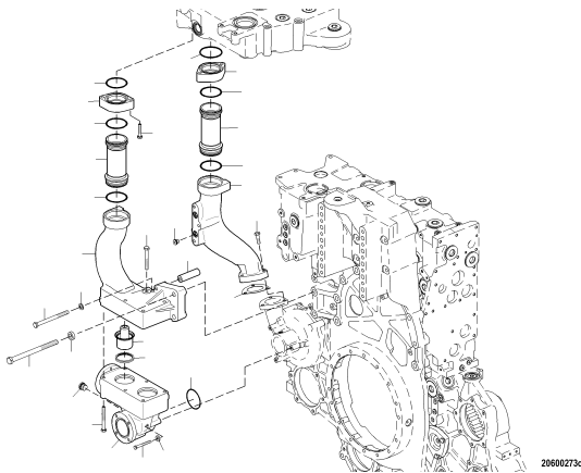
THERMOSTAT HSG LOW TEMP CIRCUIT W/TRUNIO UPC.06K06A0021
