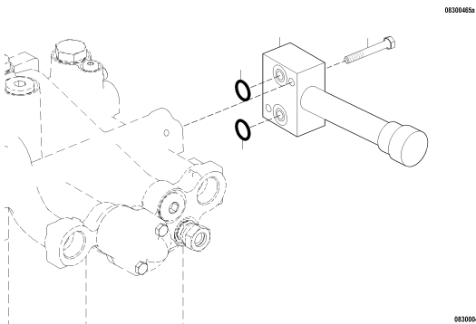
FUEL PRIMING PUMP 12/16V4000 080.00095 UPC.06M09B0006
