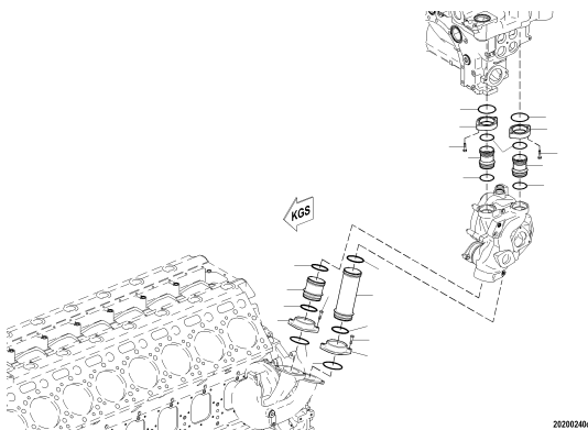
THERMOSTAT HSG HIGH TEMP CIRCUIT S4000 2 UPC.06K06B0005
