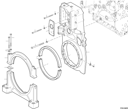
MT ENG TRUNNION 3 POINT S4000 XS526230.0 UPC.06Q00 1212
