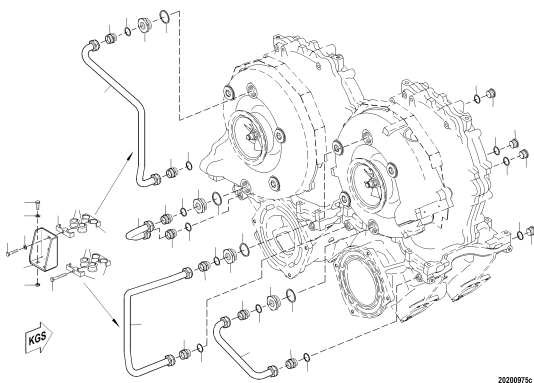
COOLANT SYS TURBO HOUSING 16V4000 X00019 UPC.06K03A0700
