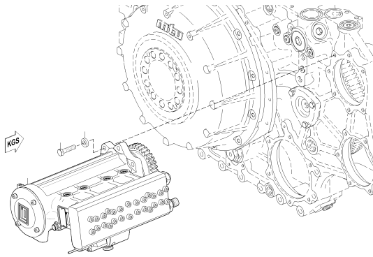
PUMP FUEL HIGH PRESS 4CYL 1800 BAR 12/16 UPC.06M04 0507
