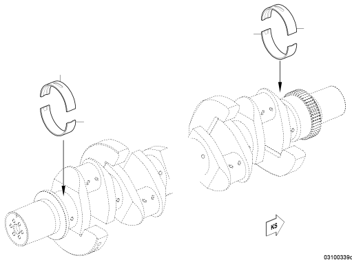
CRANKSHAFT MAIN BEARING 16V4000-03 X0001 UPC.06C01B0100
