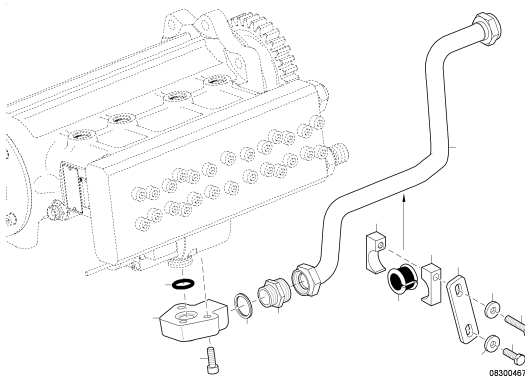
FUEL RETURN LINE LOW PRESSURE 12/16V4000 UPC.06M09F0021
