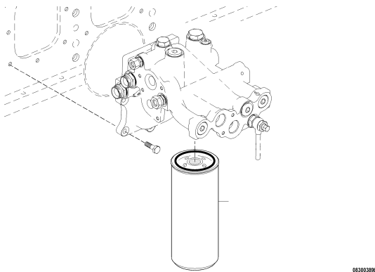
FUEL FILTER SECONDARY S4000 XS526080.000 UPC.06M09K0003
