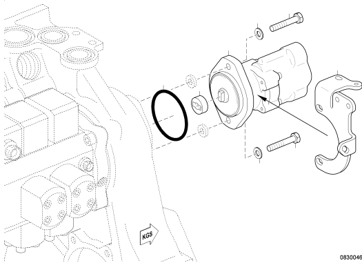
PUMP FUEL LOW PRESSURE 12/16V4000 X00040 UPC.06M04B0037
