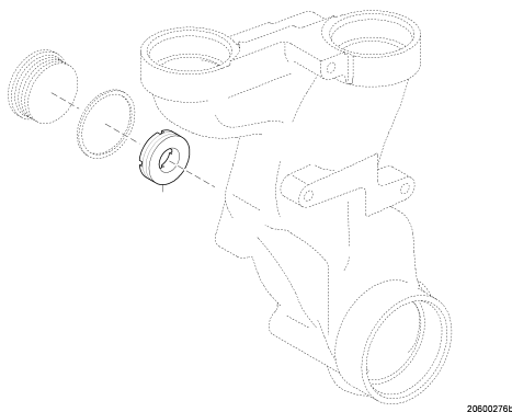
RESTRICTOR FLOW M52X1.5 X 26 X 15 16V400 UPC.06K06C0005
