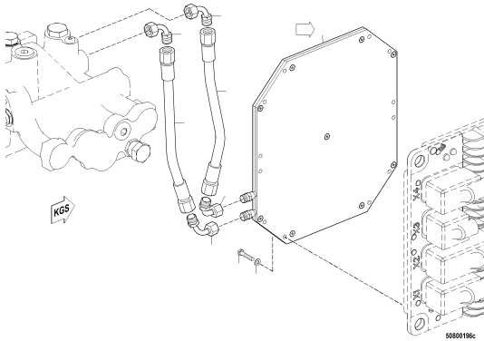
FUEL ECM COOLER S4000 ADEC X00019362 UPC.06M09G0005
