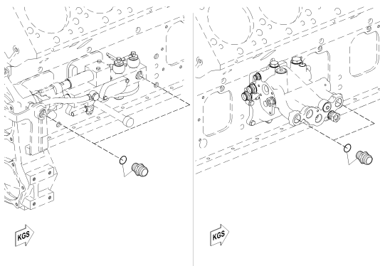
FUEL LINE UPC.06M09J0002
